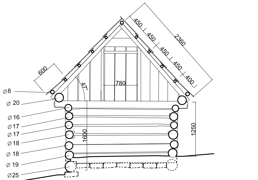
Rez AA
