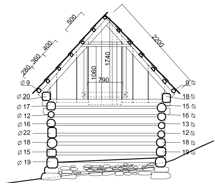
Rez AA
