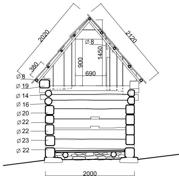
Rez AA
